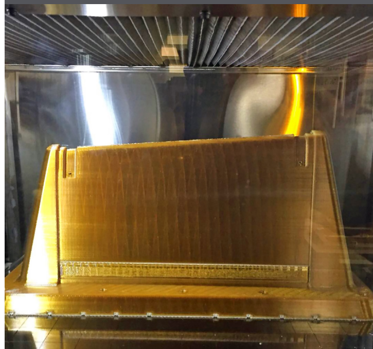
The preform tool produced with the Stratasys F900 Production System using ULTEM™ 1010 resin.
